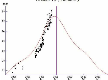
C/2020 T2 ( Palomar )
